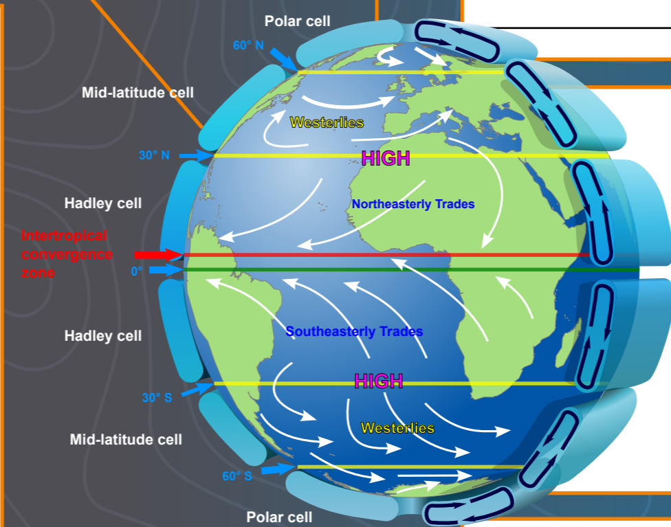
Global circulation of air
